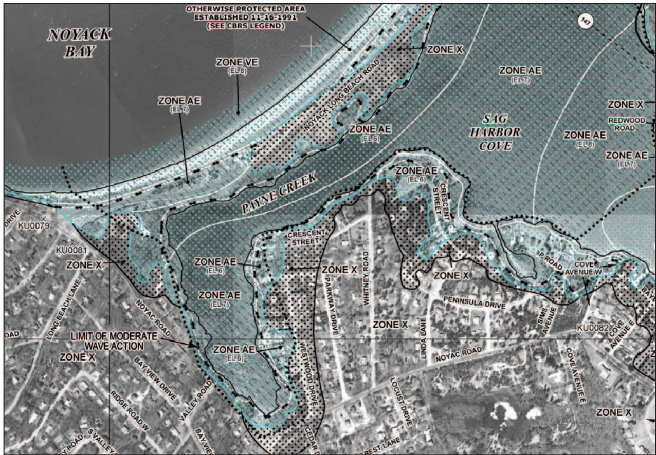
Figure 2-2. Typical DFIRM for coastal flooding showing the Limit of Moderate Wave Action (LimMA)
